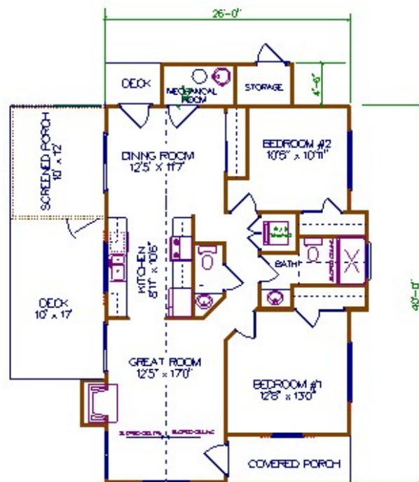
Floor Plan 992 s.f.
